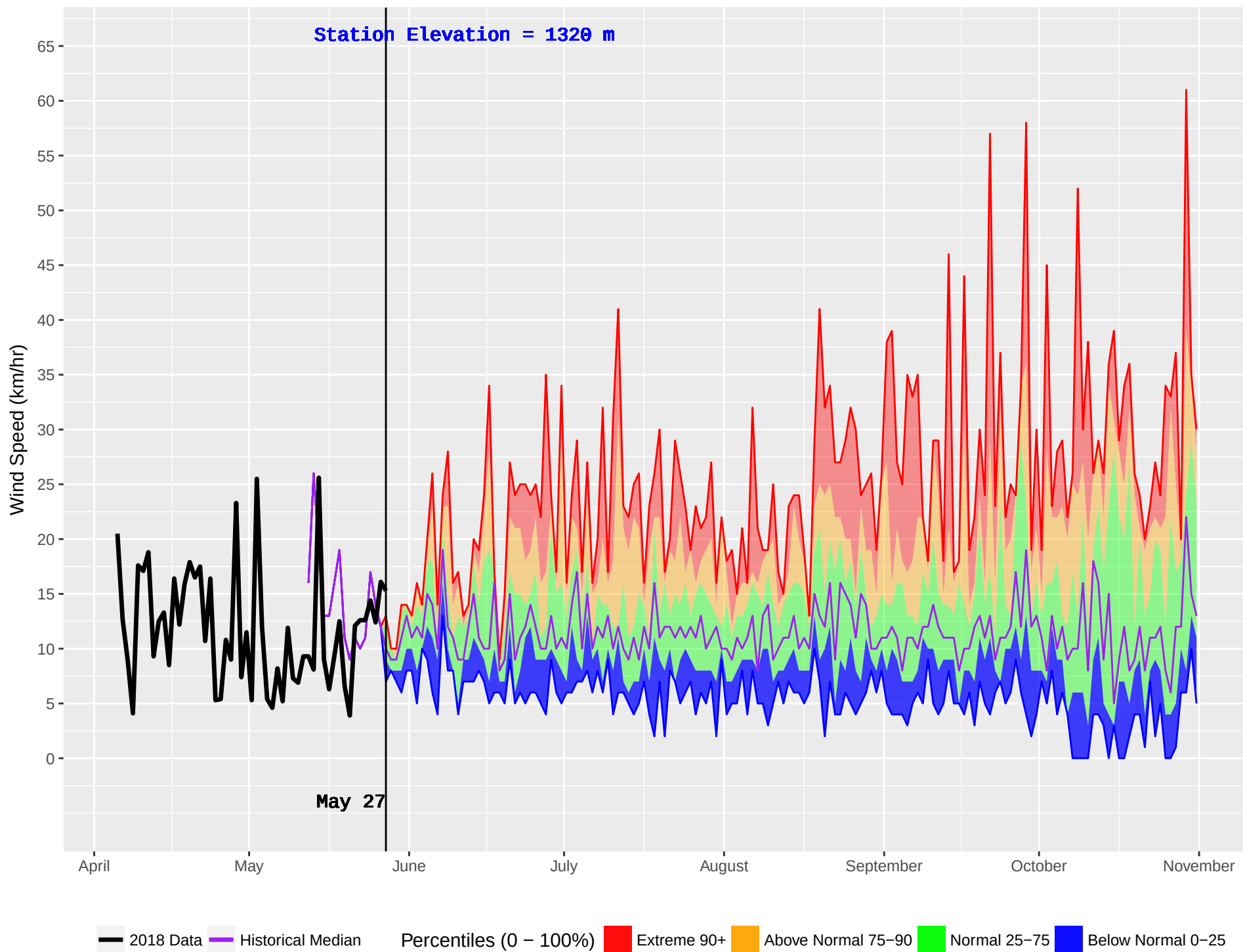
PINE CREEK (938) : Historical (2006–2016) and Current (2018) Noon Wind Speed
