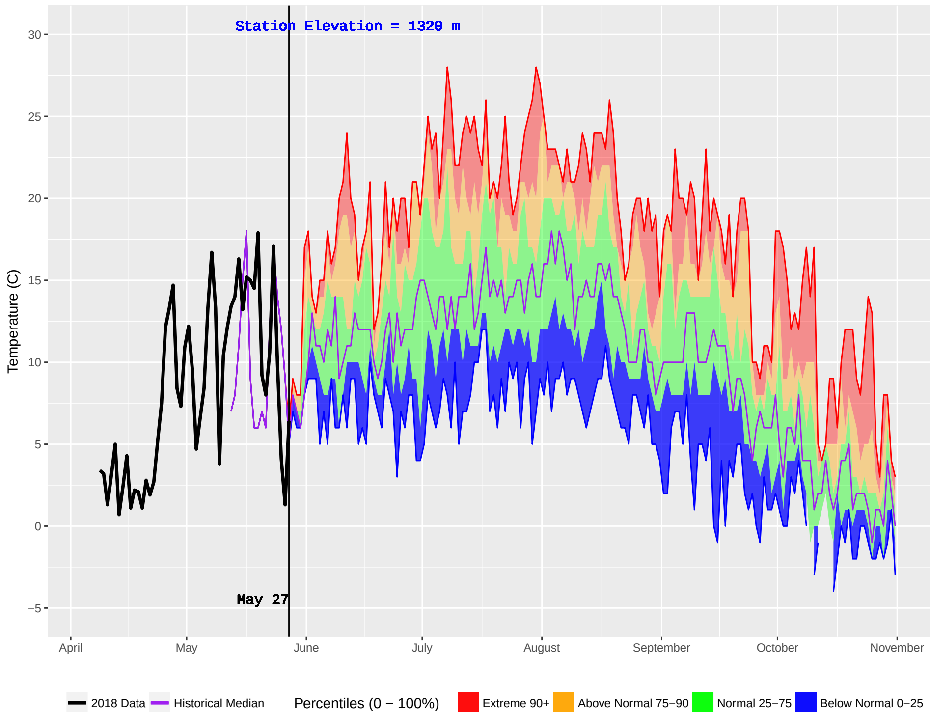
PINE CREEK (938) : Historical (2006–2016) and Current (2018) Noon Temperature
